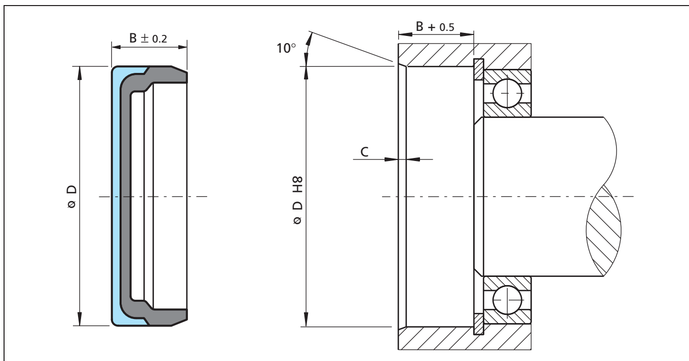
Figure 45 Installation drawing
