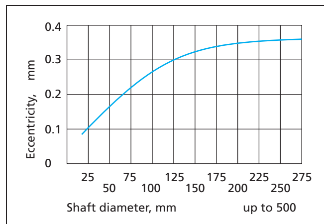
Figure 3 Eccentricity
