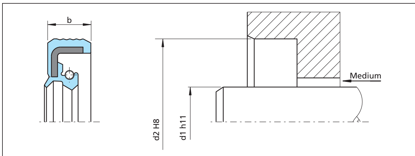
Figure 23 Installation drawing
