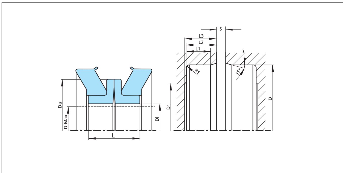
Figure 150 Installation Drawing
