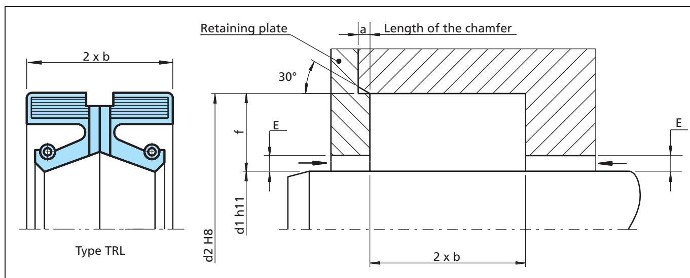
Figure 42 Installation drawing
