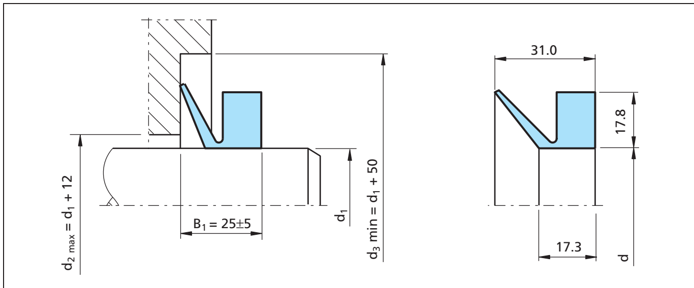
Figure 71 Installation drawing
