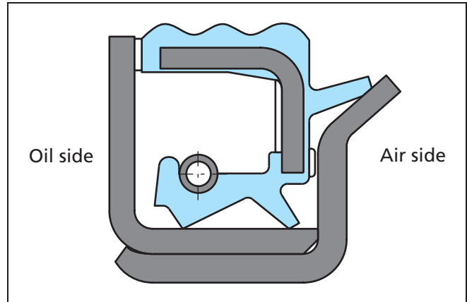
Figure 53 System 5000
