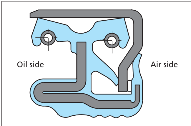
Figure 52 System 3000
