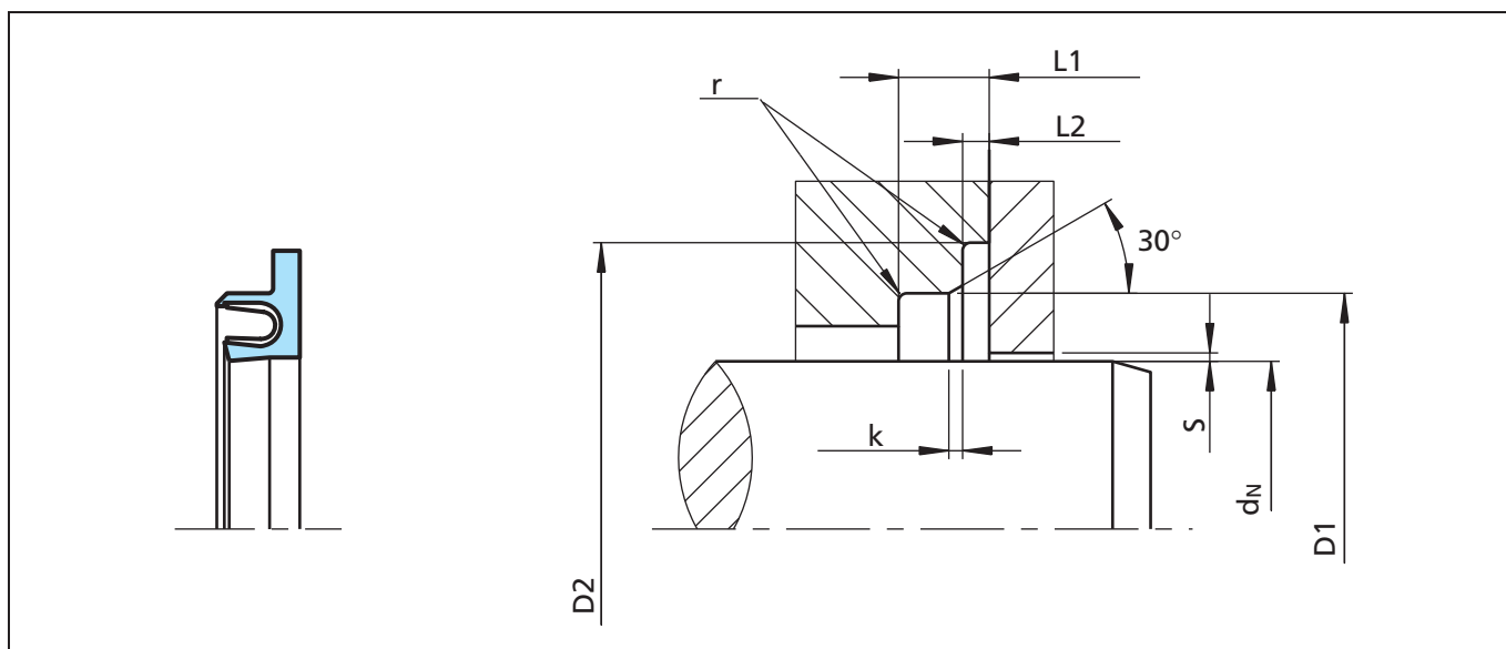
Figure 139 Installation drawing
