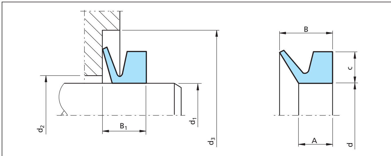
Figure 67 Installation drawing
