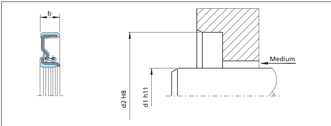
Figure 32 Installation drawing
