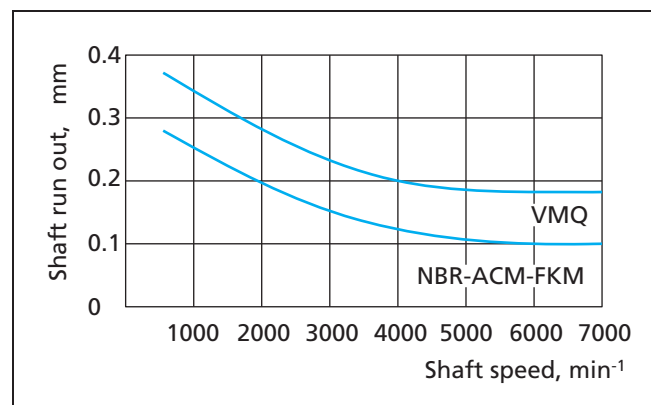
Figure 2 Shaft run out
