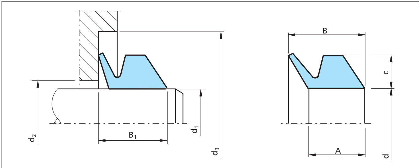
Figure 68 Installation drawing
