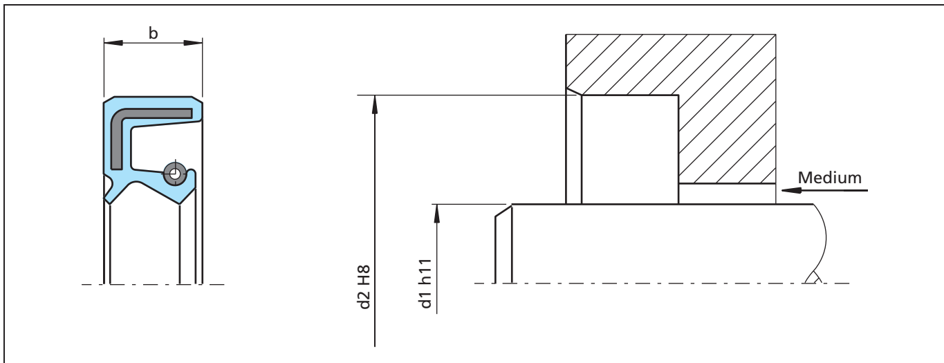
Figure 15 Installation drawing
