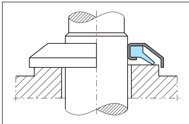
Figure 74 Vertical installation
