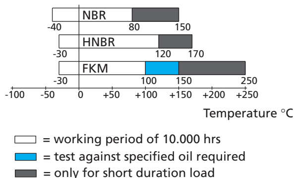
Figure 55 Temperature recommendations in typical hypoid oils
