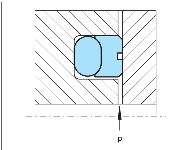
Figure 122 Axial acting Turcon® Roto Glyd Ring®
