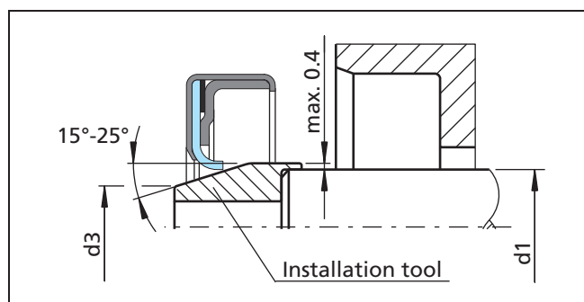
Figure 104 Fitting the sealing lip using an installation tool
