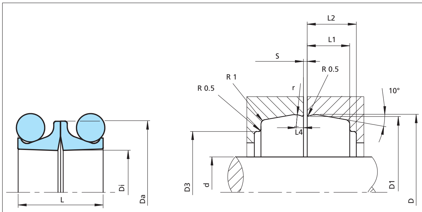
Figure 148 Installation Drawing
