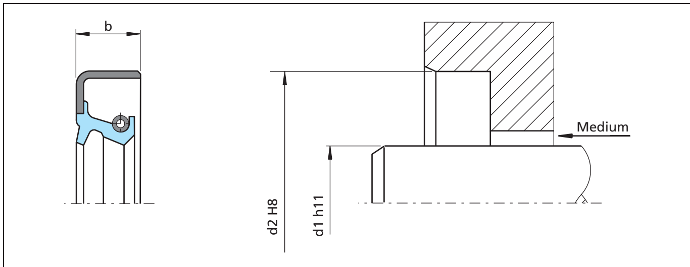
Figure 17 Installation drawing
