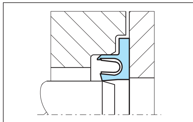
Figure 138 Turcon® Roto Variseal®
