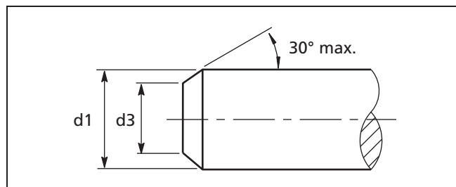
Figure 103 Shaft lead-in chamfer
